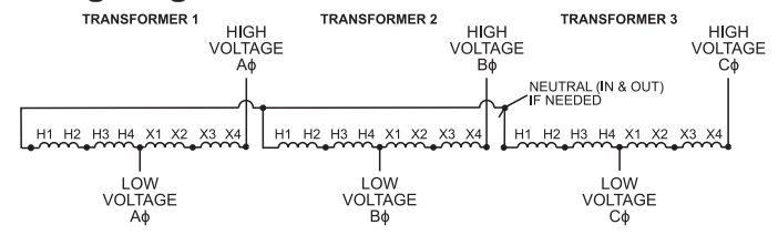
Wiring Diagram 8
