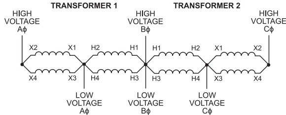
Wiring Diagram 11
