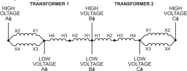
Wiring Diagram 11
