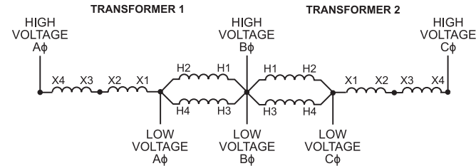
Wiring Diagram 12
