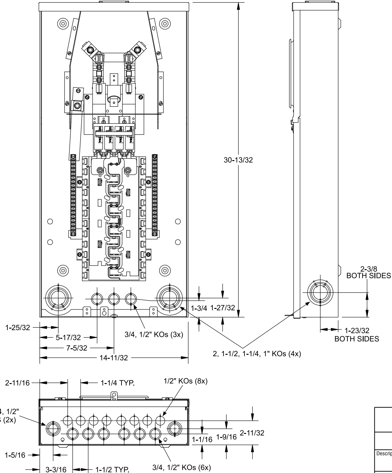
View Shown Without Covers and Deadfront
