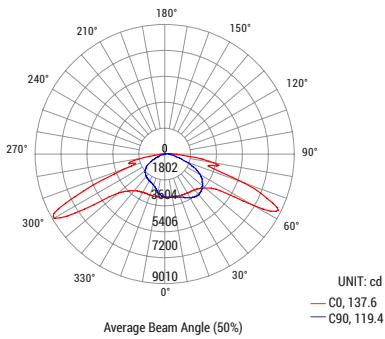
PT-AL1-100W
